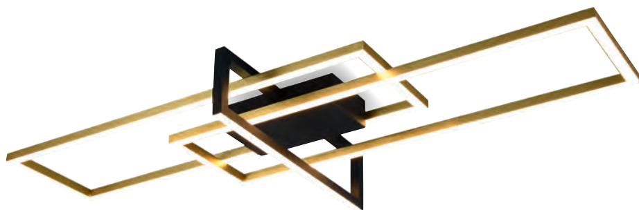
TRIO LED-Deckenleuchte messing Kunststoff weiß LxBxH: 40x100x11,5cm 1xSMD inkl. LED 34W 3.000K 3.900lm
