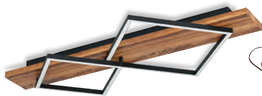
EGLO LED-Deckenleuchte Stahl Holz rustikal schwarz braun LxBxH: 78x40,5x9cm inkl. LED 1x13W+1x15W 3.000K 1.750+2.000lm
